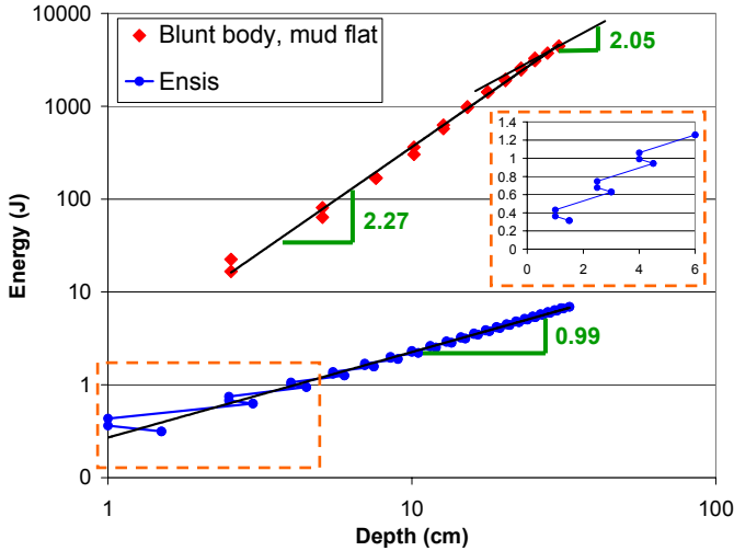
Figure 2. Ensis vs. blunt body energy expenditure
